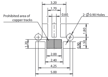
P.C.B MOUNTING SOLDER LAND DIMENSION
